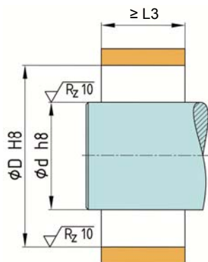
Space Surface quality and tolerances
